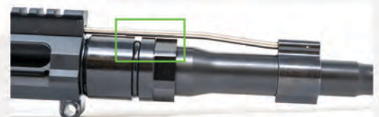
FAXON AR-10 GAS BLOCK ENHANCED CLEARANCE BETWEEN GAS TUBE AND BARREL NUT
